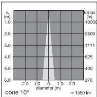
100w 10° lamp
