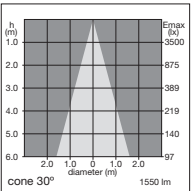
100w 30° lamp
