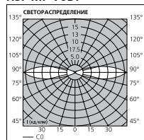
HSI-MP 70Вт
