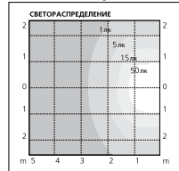
Borneo 100 Lynx-S 11Вт
