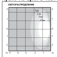
Rytmo AS Lynx-D 18Вт
