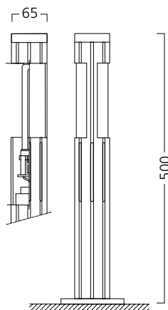
Столбик XS 11Вт
