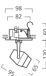
XS BriteSpot ES50
