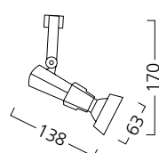
XS Hi-Spot ES50
