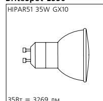
BriteSpot ES50
