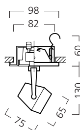
XS Superia 50
