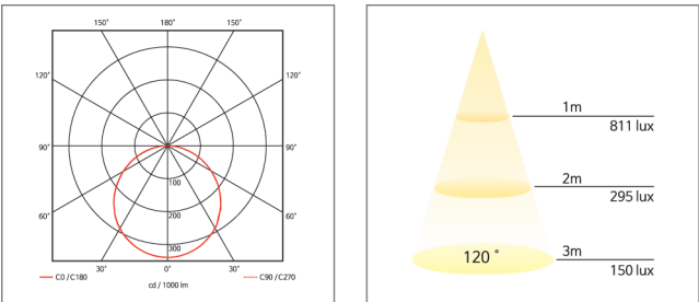
ILLUMINATION_Photometric Data
