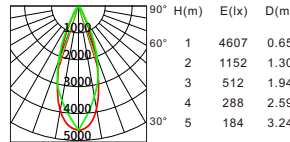
Beam angle:36° Luminous flux:1762lm
