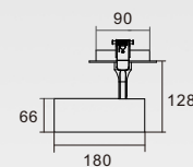
KAS-TL10L-C-66 Power: 10W/15W Diameter: 66mm Cutout: 85-90mm
