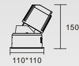
K-CL36-4T-S1D Power: 20W/25W Cutout: 100*100mm Height: 150mm
