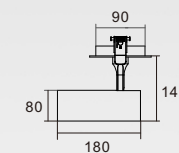
KAS-TL10R-C-80 Power: 25W/30W Diameter: 80mm Cutout: 85-90mm
