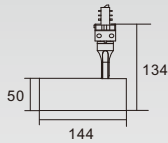
KAS-TL10L-A-50 Power: 7W Diameter: 50mm
