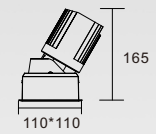
K-CL36-4T-S1D Power: 30W Cutout: 100*100mm Height: 165mm
