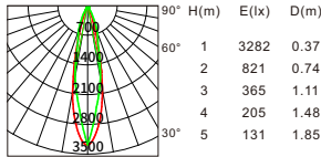
Beam angle:24° Luminous flux:581lm
