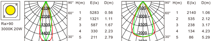
Beam angle:30° Luminous flux:1592lm Beam angle:60° Luminous flux:1724lm
