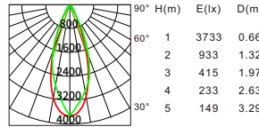
Beam angle:36° Luminous flux:1472lm
