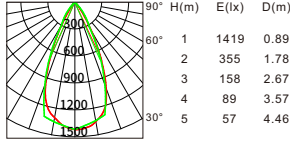
Beam angle:50° Luminous flux:855lm
