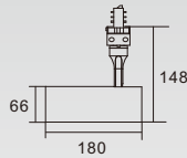
KAS-TL10L-A-66 Power: 10W/15W Diameter: 66mm
