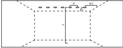
Model: 35W A:800mm B:1000mm H:3000mm
