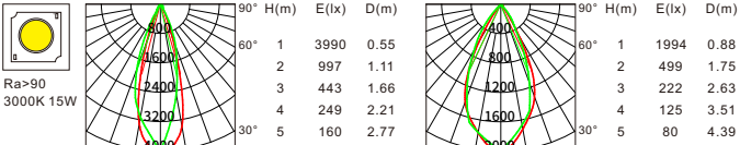
Beam angle:30° Luminous flux:1197lm Beam angle:50° Luminous flux:1236lm
