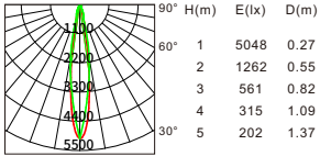
Beam angle:18° Luminous flux:551lm
