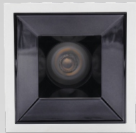
K-CL36-3F-S1D Power: 5W/8W Cutout: 75*75mm Height: 90mm
