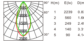
Beam angle:45° Luminous flux:1329lm
