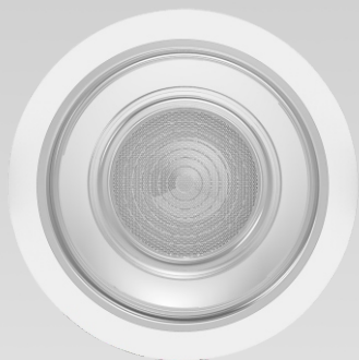
KS-DL07L-B-7 Power: 35W/40W/45W Cutout: 175mm Height: 121mm
