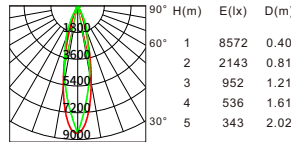
Beam angle:24° Luminous flux:1797lm
