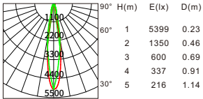
Beam angle:15° Luminous flux:462lm
