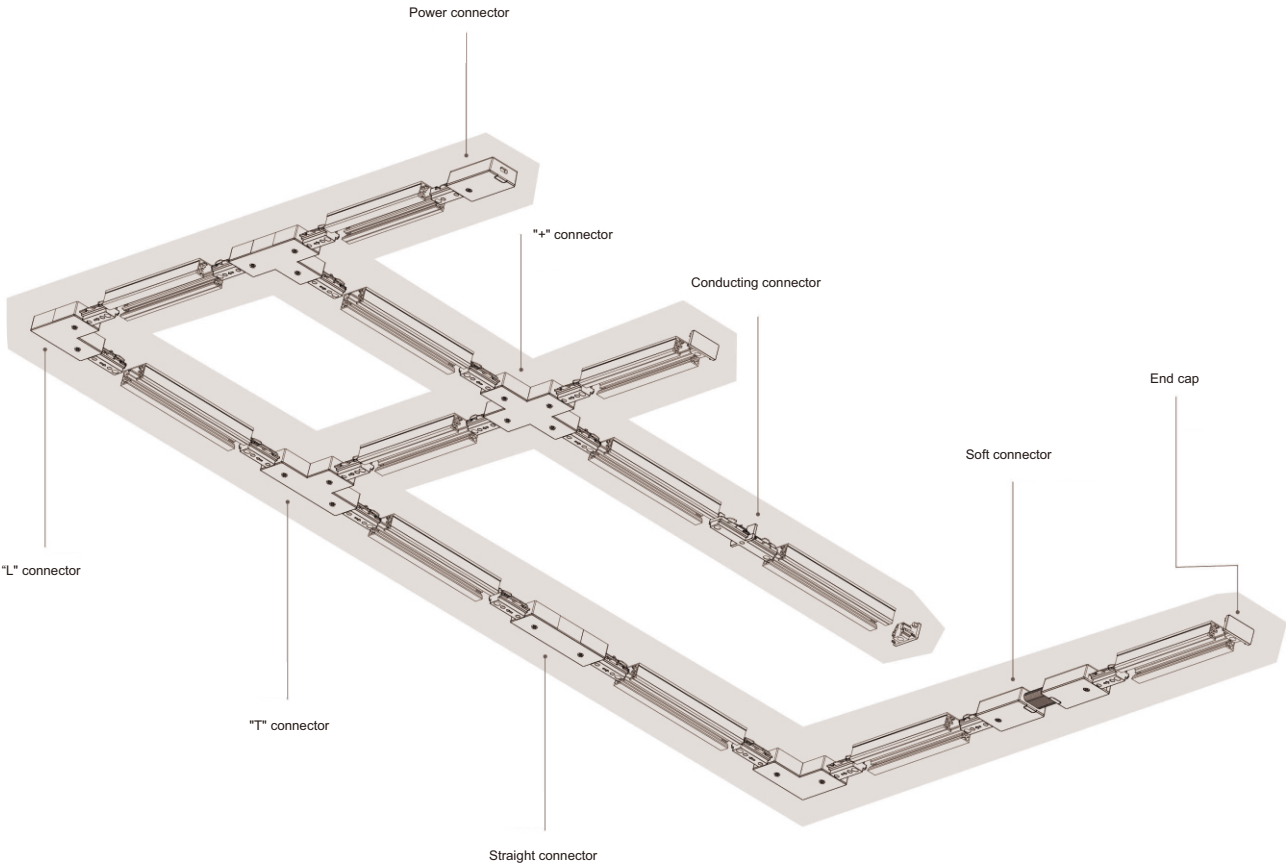
Reference Diagram for choice of connectors
