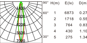
Beam angle:15° Luminous flux:1097lm
