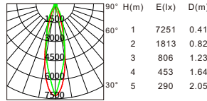
Beam angle:24° Luminous flux:1561lm
