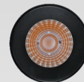
KAS-TL10L-C-80 Power: 25W/30W Diameter: 80mm Cutout: 85-90mm
