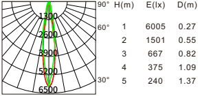
Beam angle:18° Luminous flux:658lm
