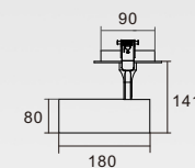
KAS-TL10L-C-80 Power: 25W/30W Diameter: 80mm Cutout: 85-90mm
