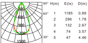
Beam angle:50° Luminous flux:713lm
