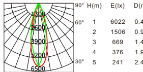
Beam angle:30° Luminous flux:1664lm
