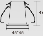
KS-BL01R-1D-04 Power: 2W Cutout: 37*37mm Height: 49mm
