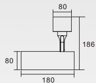
KAS-TL10R-D-80 Power: 25W/30W Diameter: 80mm
