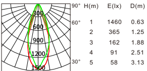
Beam angle:36° Luminous flux:545lm
