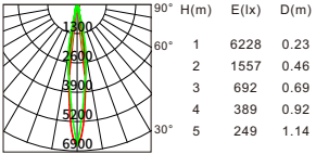
Beam angle:15° Luminous flux:533lm
