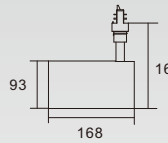
KAS-TL10R-A-93 Power: 25W/30W Diameter: 93mm
