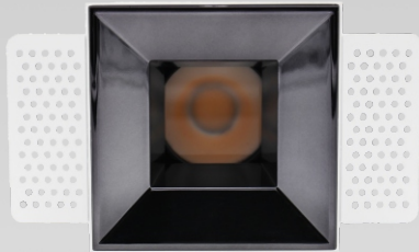
K-CL36-4F-S3D Power: 20W/25W Cutout: 100*100mm Height: 150mm
