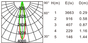
Beam angle:18° Luminous flux:430lm
