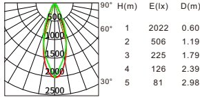
Beam angle:36° Luminous flux:710lm
