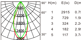
Beam angle:45° Luminous flux:1657lm
