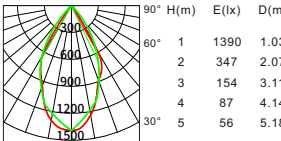
Beam angle:60° Luminous flux:1049lm
