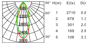
Beam angle:30° Luminous flux:1408lm
