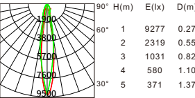
Beam angle:15° Luminous flux:1482lm
