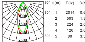
Beam angle:30° Luminous flux:1045lm
