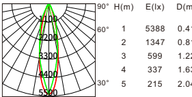
Beam angle:24° Luminous flux:1347lm
