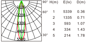
Beam angle:24° Luminous flux:881lm
