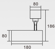
KAS-TL10L-D-80 Power: 25W/30W Diameter: 80mm
