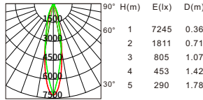
Beam angle:18° Luminous flux:1293lm
