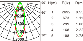
Beam angle:36° Luminous flux:976lm
