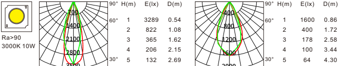
Beam angle:30° Luminous flux:934lm Beam angle:50° Luminous flux:975lm
