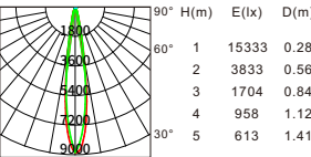
Beam angle:15° Luminous flux:1731lm
