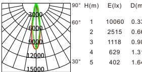
Beam angle:20° Luminous flux:1662lm
