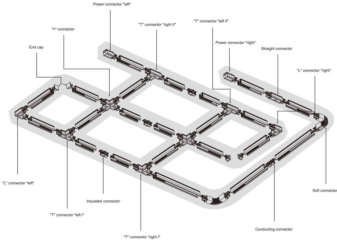
Reference Diagram for choice of connectors
