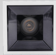
K-CL36-3T-S1D Power: 10W/12W Cutout: 75*75mm Height: 110mm
