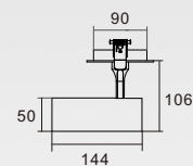
KAS-TL10L-C-50 Power: 7W Diameter: 50mm Cutout: 85-90mm
