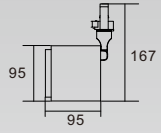
KAS-TL18-C-95 Power: 20W/30W Diameter: 95mm
