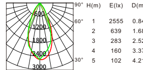
Beam angle:45° Luminous flux:1549lm
