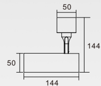
KAS-TL10L-D-50 Power: 7W Diameter: 50mm
