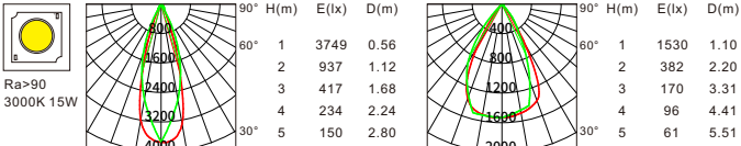
Beam angle:30° Luminous flux:1142m Beam angle:60° Luminous flux:1250lm
