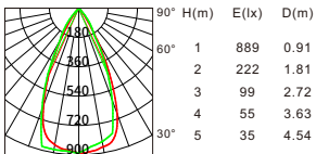
Beam angle:50° Luminous flux:562lm
