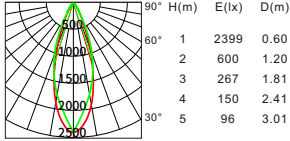
Beam angle:36° Luminous flux:847lm
