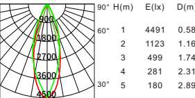
Beam angle:36° Luminous flux:1669lm
