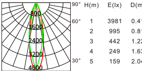
Beam angle:24° Luminous flux:997lm
