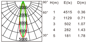
Beam angle:24° Luminous flux:744lm
