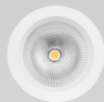
KAS-DL03-R-6 Power: 20W/30W/40W Cutout: 160-175mm Height: 80mm
