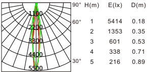
Beam angle:11° Luminous flux:336lm
