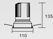
K-CL36-4W-R1S Power: 30W Cutout: 100mm Height: 135mm
