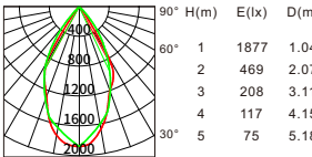
Beam angle:60° Luminous flux:1418lm
