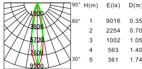
Beam angle:18° Luminous flux:1529lm
