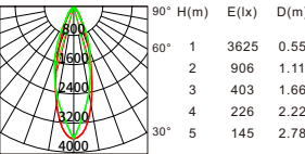
Beam angle:36° Luminous flux:1317lm
