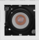
KAS-BL10R-1-3 Power: 10W Cutout: 82*82mm Height: 106.5mm
